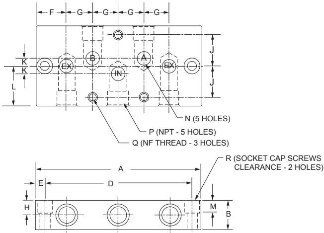
SIDE-PORTED
