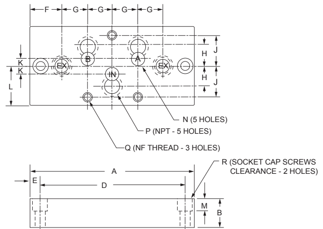
BOTTOM PORTED
