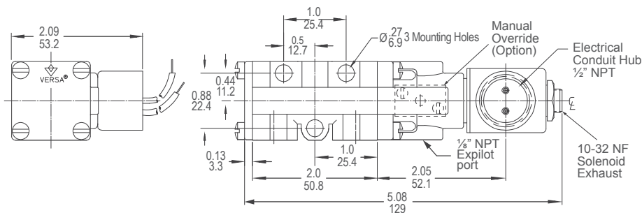
EXPilot type BSG-3303-316-(* )
